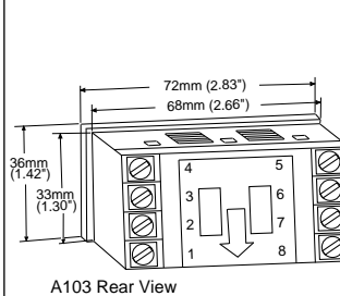
Option Module Rear View
